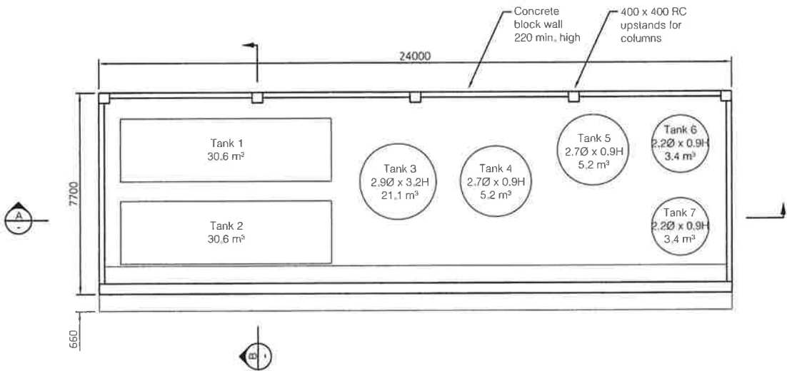
Liquid Store Layout (Scale A)
