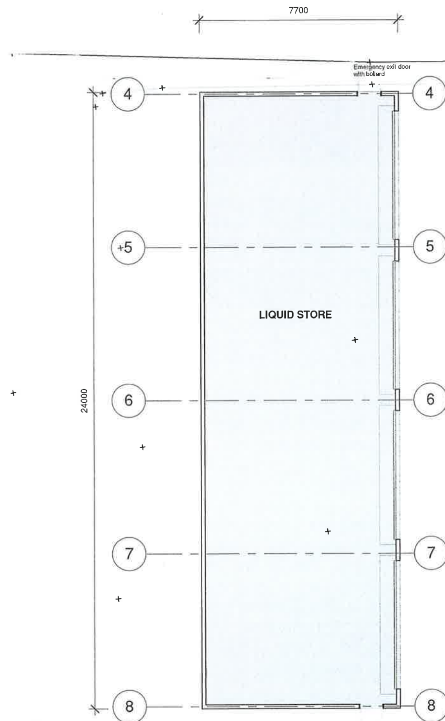
1 LIQUID STORE 1 : 100
