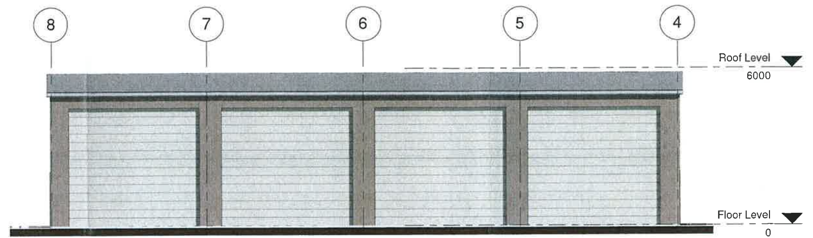
2 Liquid Store Front Elevation 1 : 100
