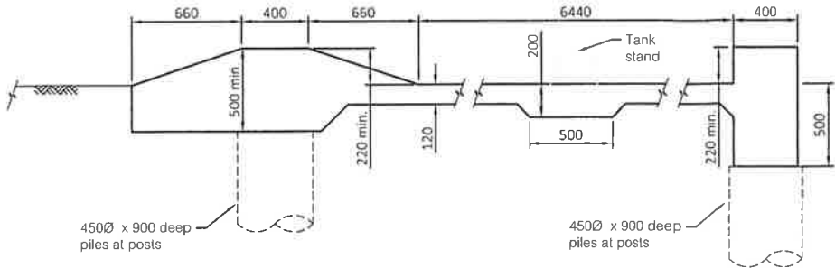
Section B-B (Scale B)
