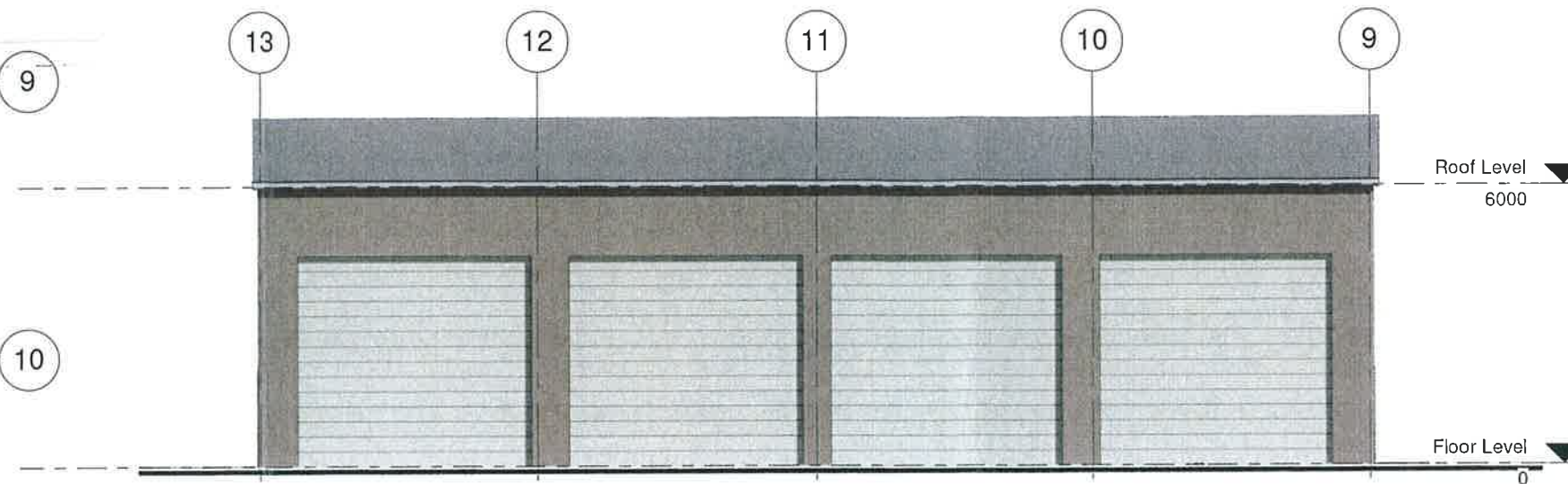
2 Elevation Storage Shed 1 : 100
